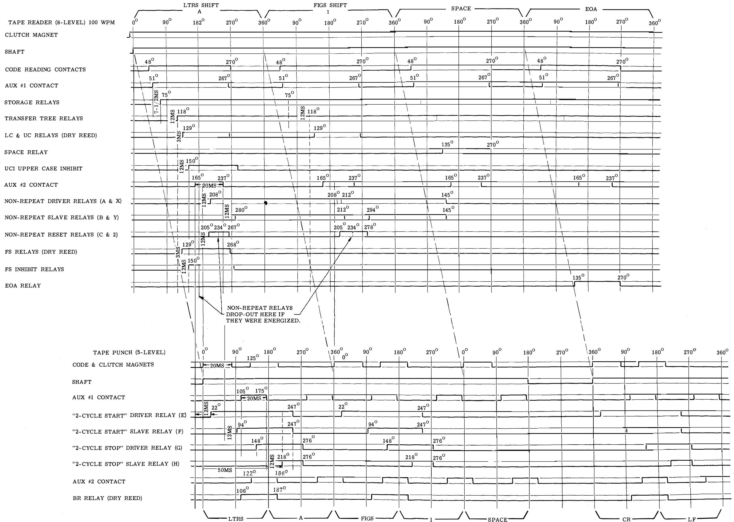
Figure 4 - Timing Diagram, Tape-to-Tape Universal Station Converter
