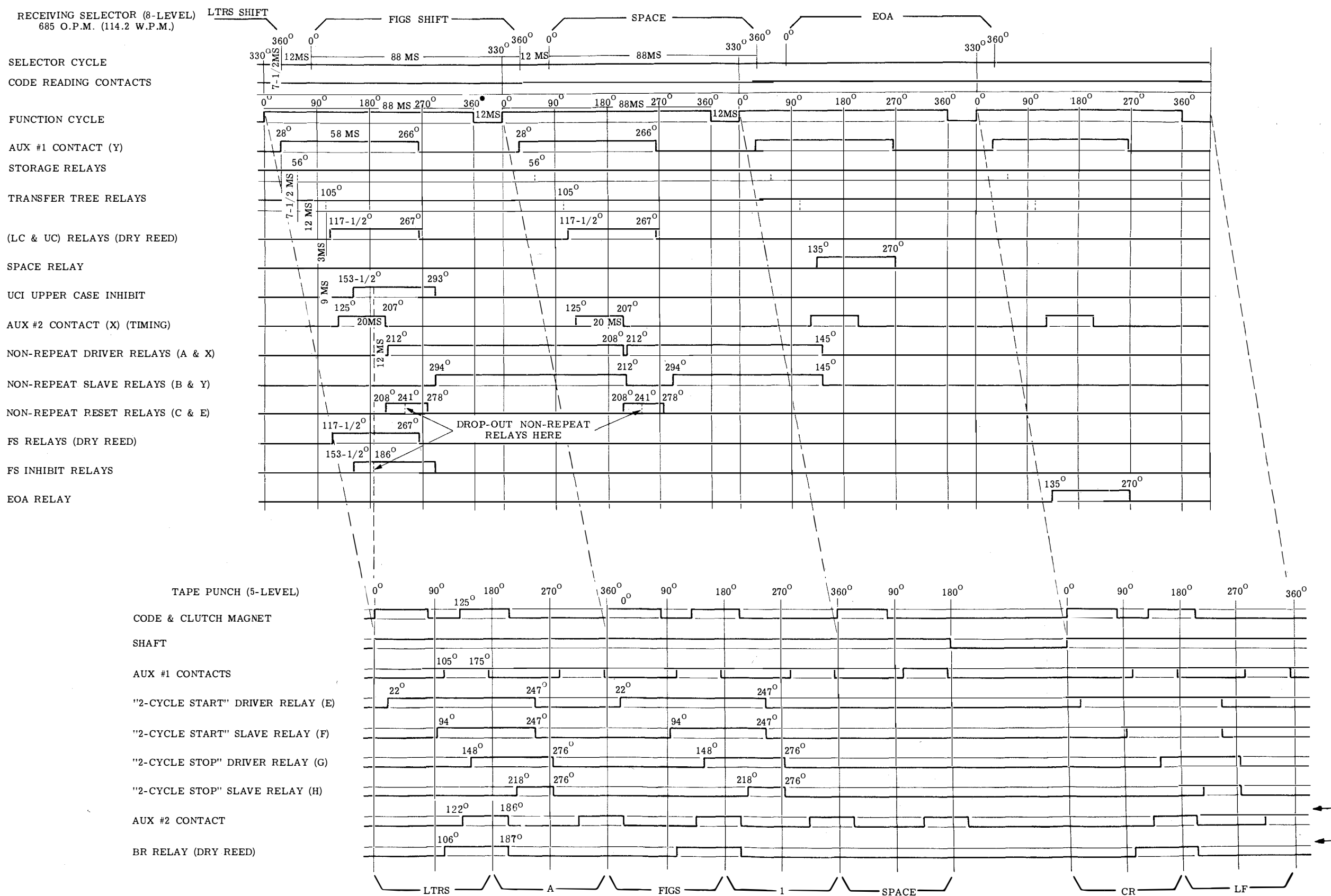
Figure 3 - Timing Diagram, Signal-to-Tape Universal Station Converter
