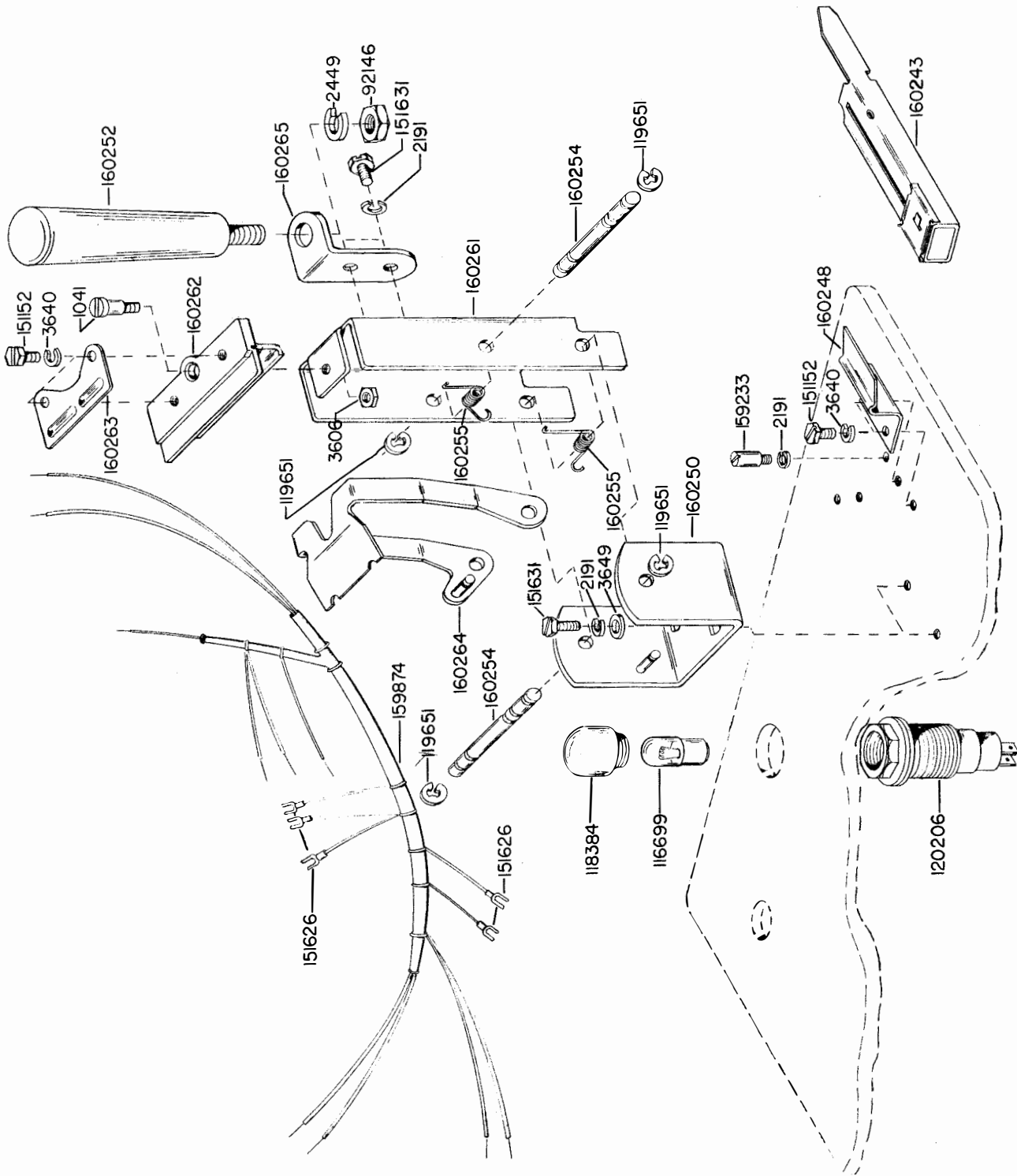
FIGURE 2. CUTTER MECHANISM AND CABLE
